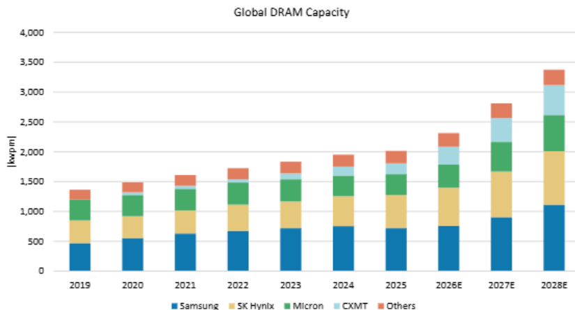
Exhibit 3: Global DRAM capacity to reach 3,374kwpm in 2028e, while CXMT may account for 15% of that (around 500kwpm by 2028)
